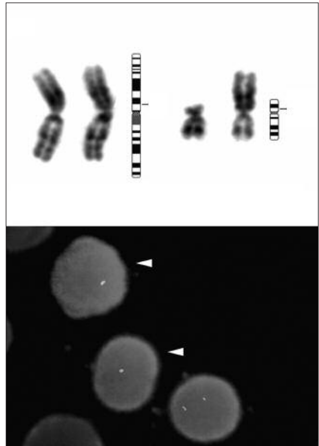
Fig 1. A) Partial karyotype showing der(17)t(1;17)(p13;p11.2). G-banding with trypsin-Giemsa. B) Interphase fluorescence in situ hybridisation analysis using the SpectrumOrange probe for TP53 on 17p13.1. A single signal in two marrow cells (arrowheads) is seen, consistent with heterozygous deletion of TP53 .
